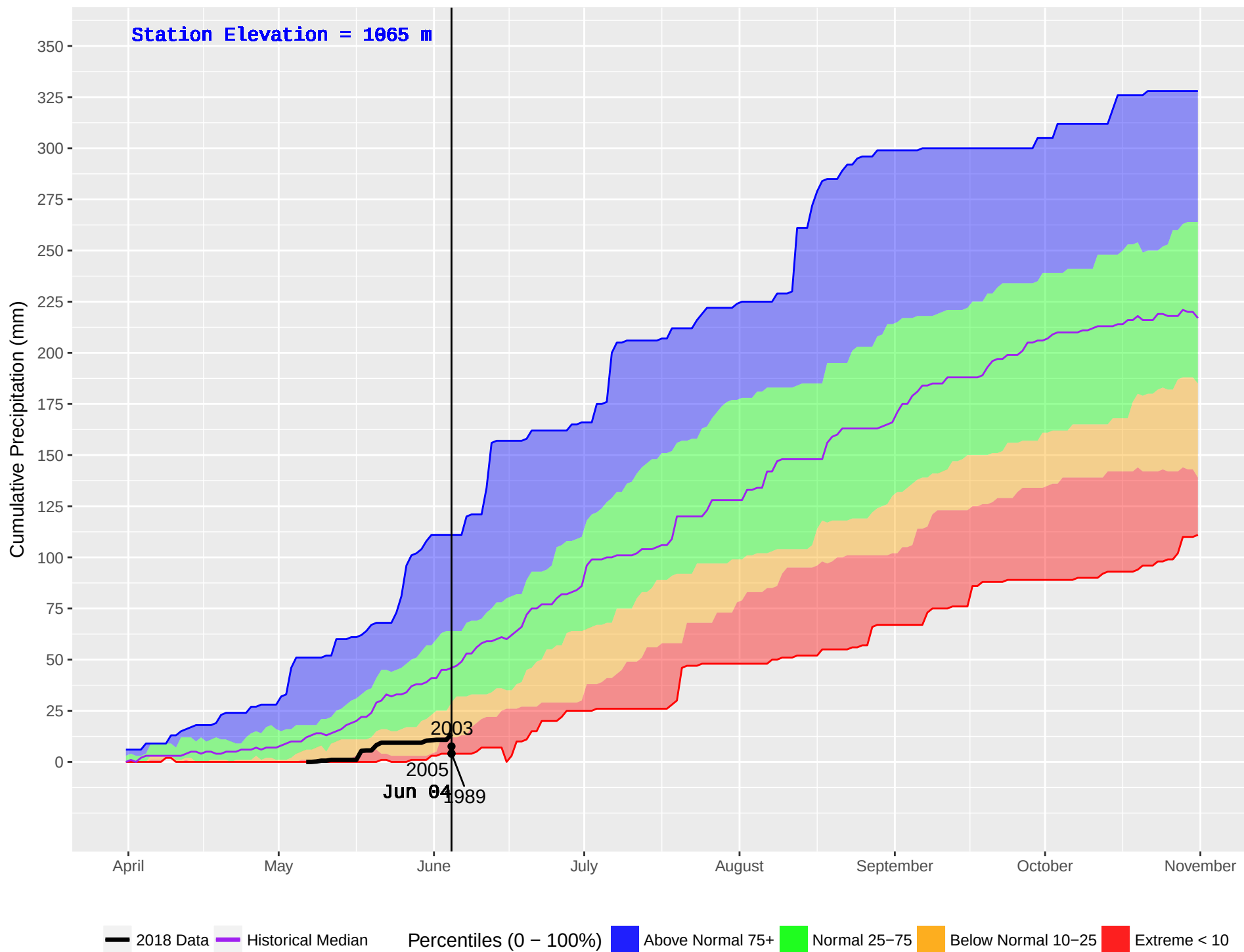
PLACE LAKE (212) : Historical (1981–2016) and Current (2018) Noon Cumulative Precipitation
