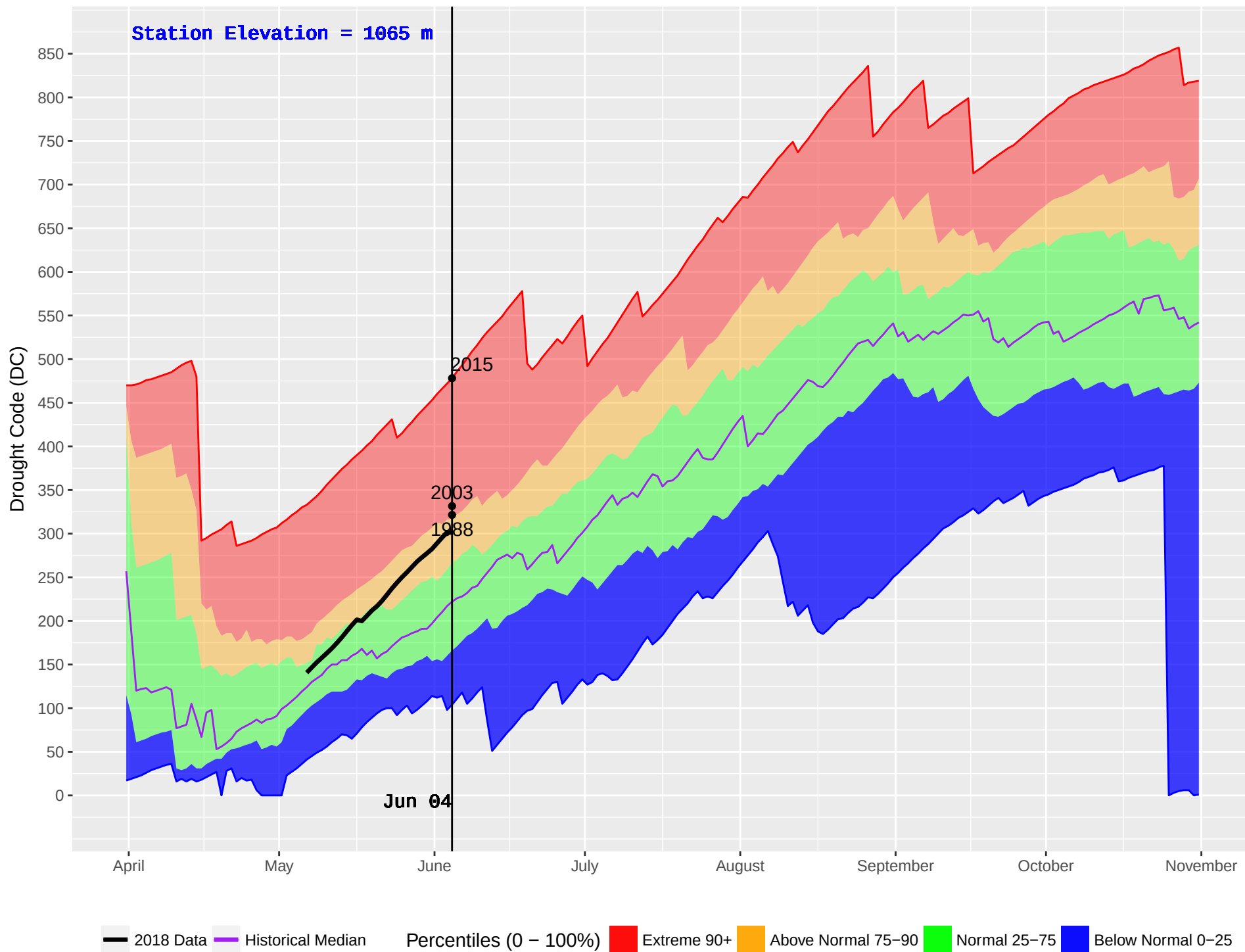
PLACE LAKE (212) : Historical (1981–2016) and Current (2018) Noon Drought Code (DC)
